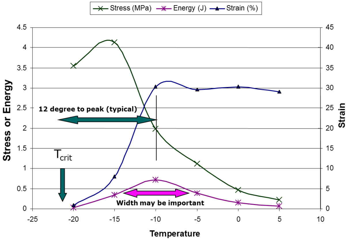
Figure 7: DTT data represented as stress, strain and energy at a break condition (Rowe and Sharrock, 2004)
