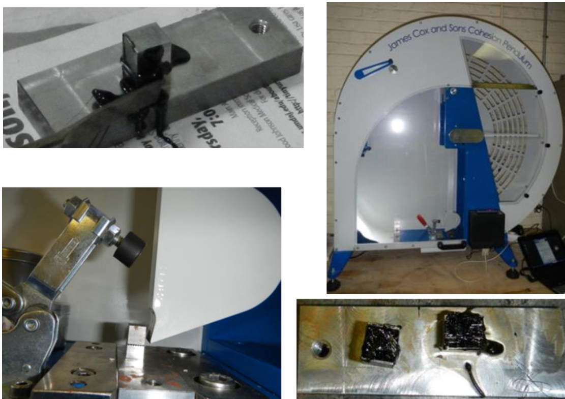
Figure 2: The Vialit pendulum test; top left – specimen preparation, bottom left – pendulum shown in position in which it would strike upper fixture of sample, top right – general view of apparatus, bottom right – fractured surfaces
