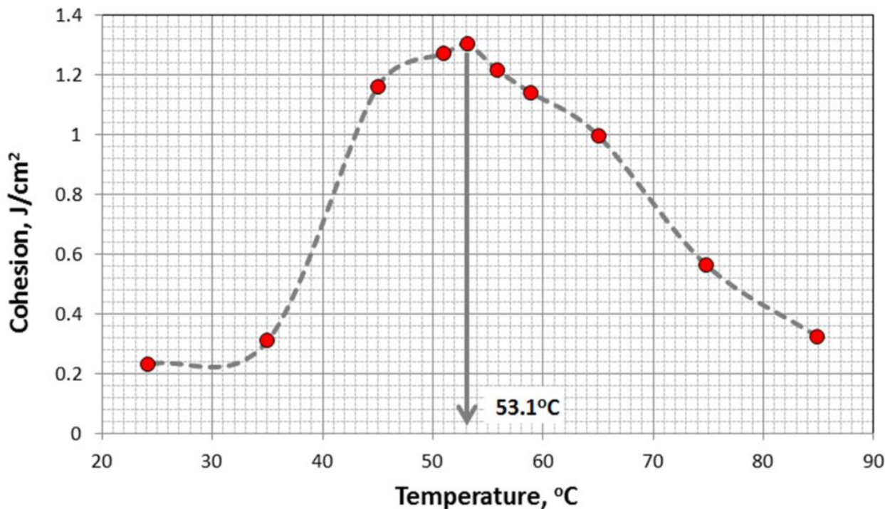
Figure 5: Cohesion versus temperature for a PG76-22 binder
