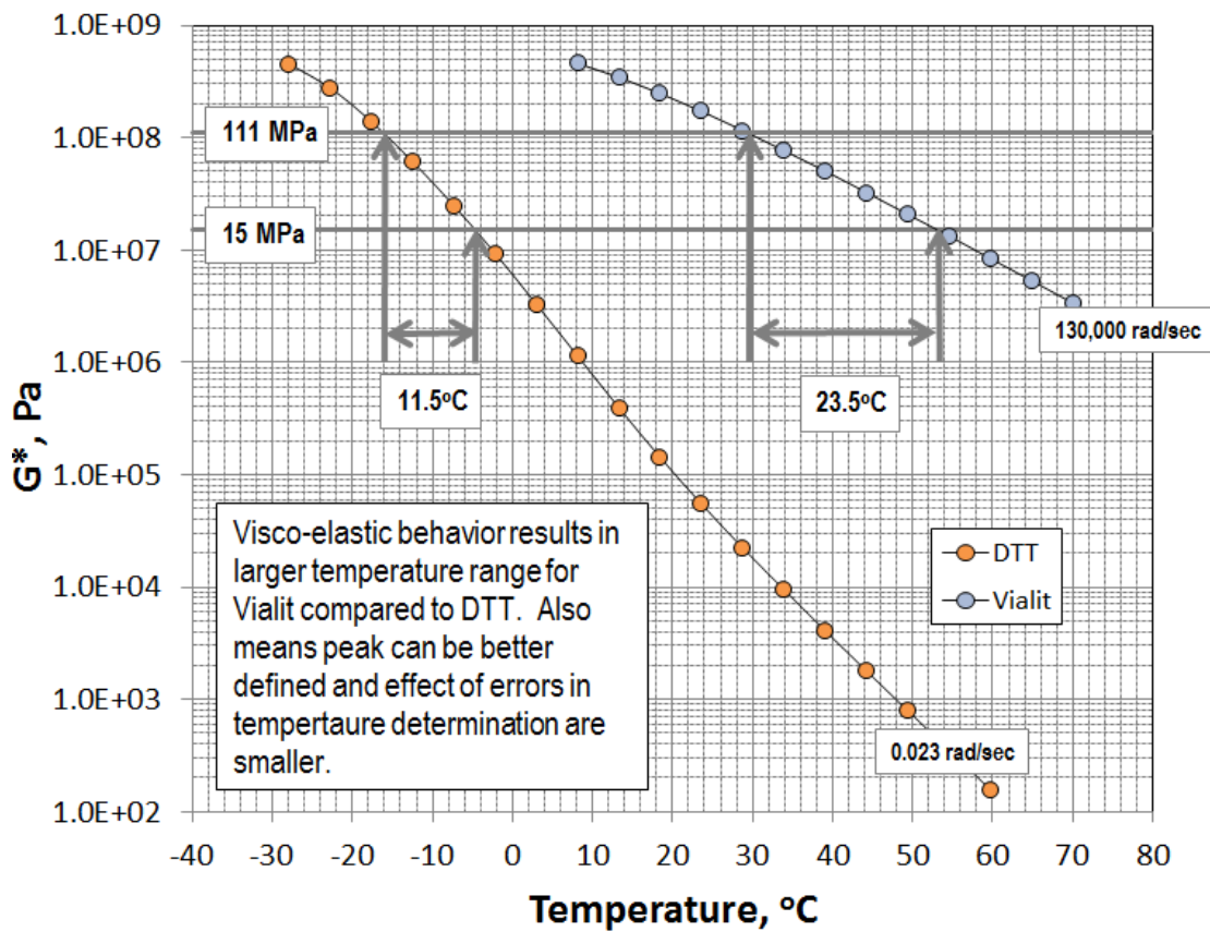
Figure 8: Computation of isochrones corresponding to loading times deduced for the DTT test and the Vialit tests
