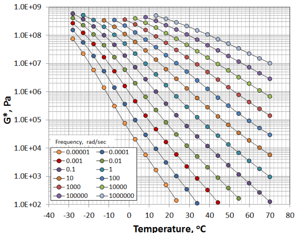
Figure 6: Isochrones of G^* produced using the relaxation spectra obtained for the PG76-22 binder
