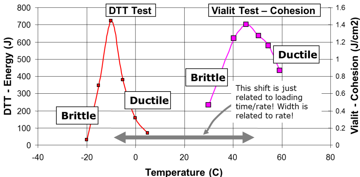
Figure 3: Comparison of Energy dissipated in a DTT fracture test versus cohesion in a Vialit Cohesion Pendulum test
