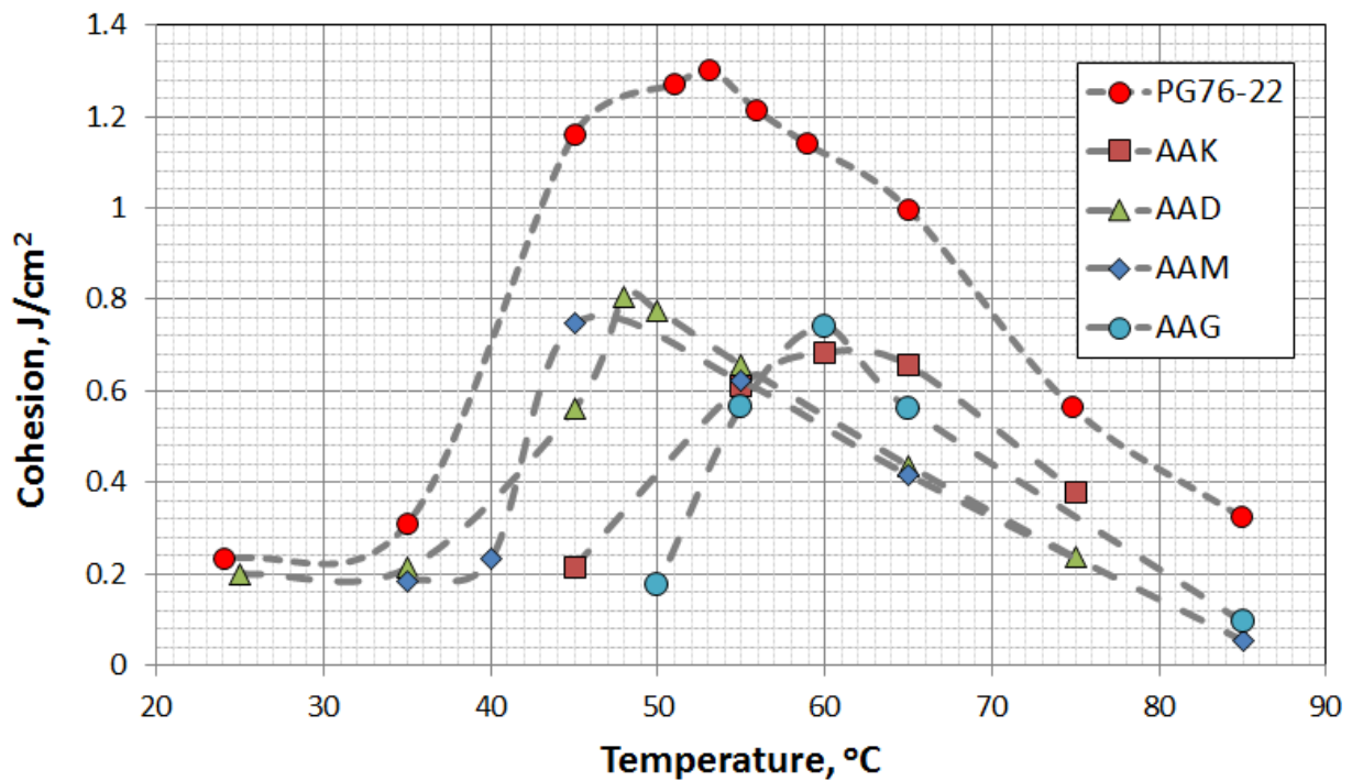
Figure 9: Comparison of a modified PG76-22 versus four SHRP PAV-aged asphalt binders in the Vialit Pendulum test
