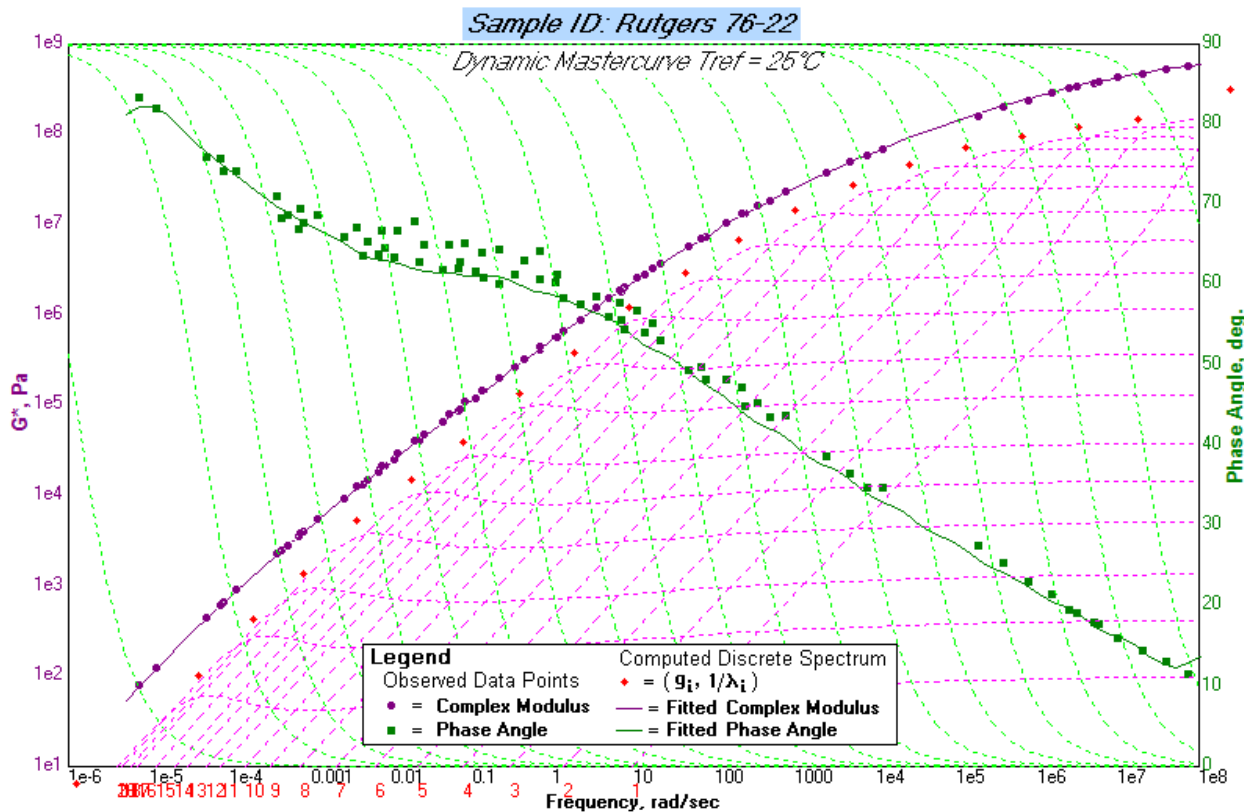
Figure 4: Master curve for PG76-22 binder at a reference temperature of 25°C
