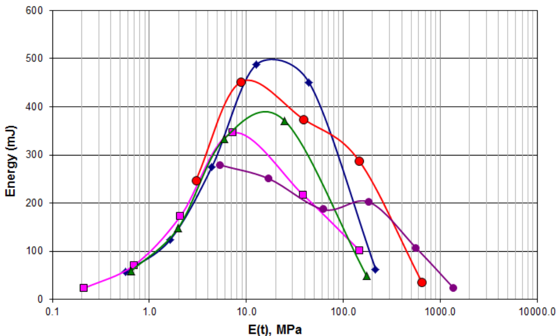
Figure 1: Data from various filled binder systems tested in the Direct Tension test with energy plotted against E(t)
